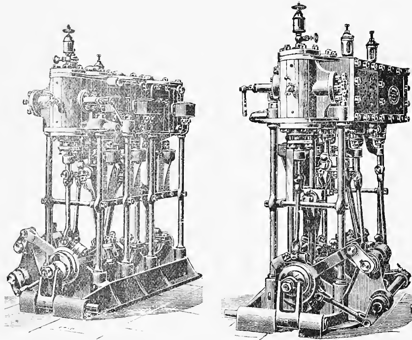
Paul's Patent Eccentric Single Valve Gear, equal to Link Motion.
